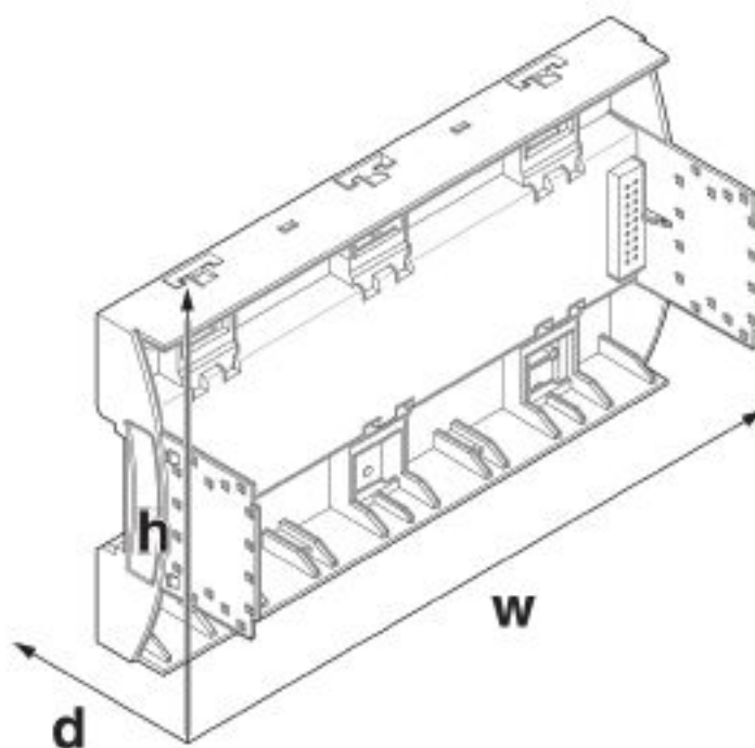
Dimensional drawing
