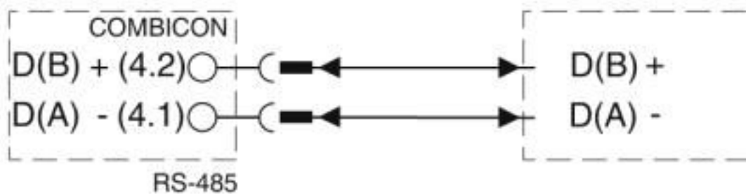
Connection diagram
