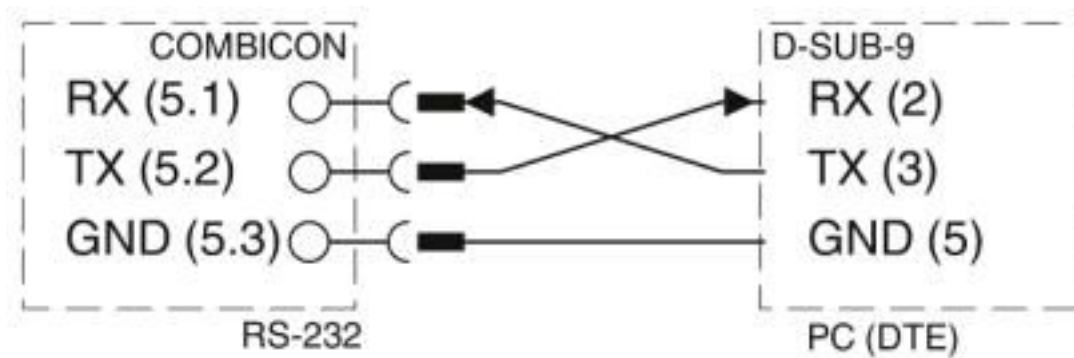
Connection diagram
