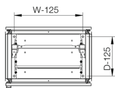
Sectional top view
