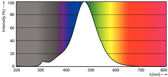
Spectral Power Distribution Colour - LEDclassic 11W A60 E27 smoky ND RFSRT4
