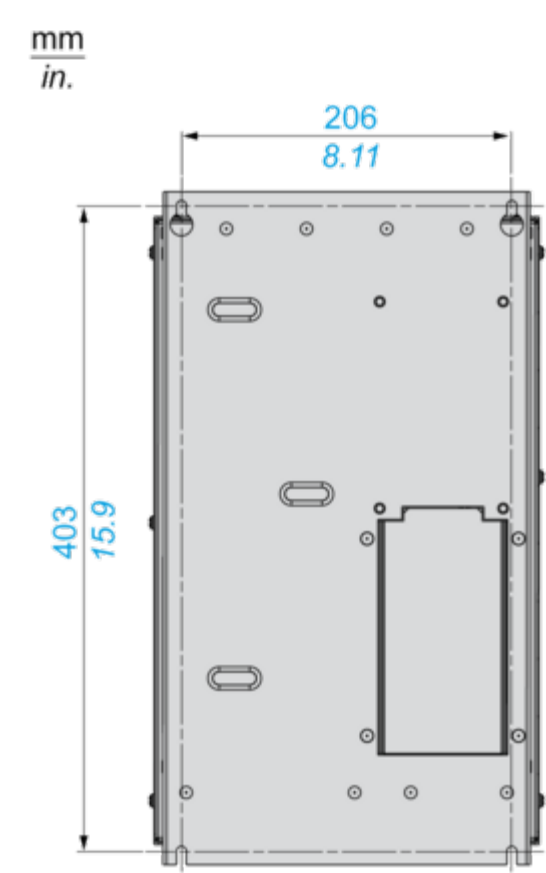
Drives with IP20 Top Cover Front, Left and Rear View
