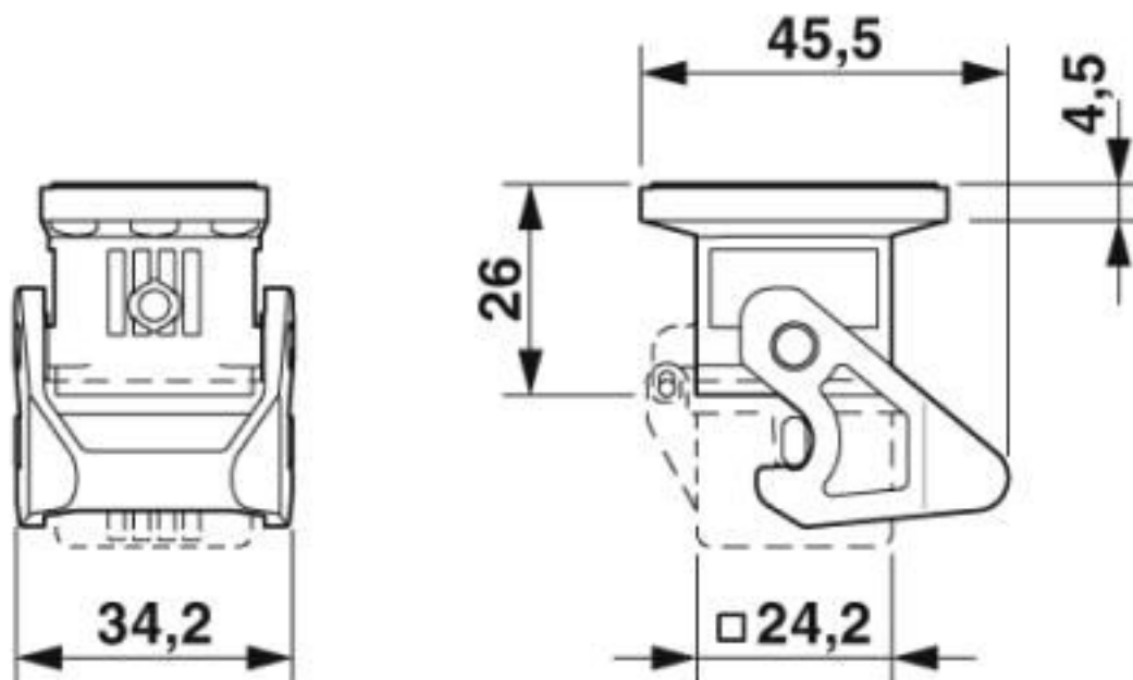
Dimensional drawing
