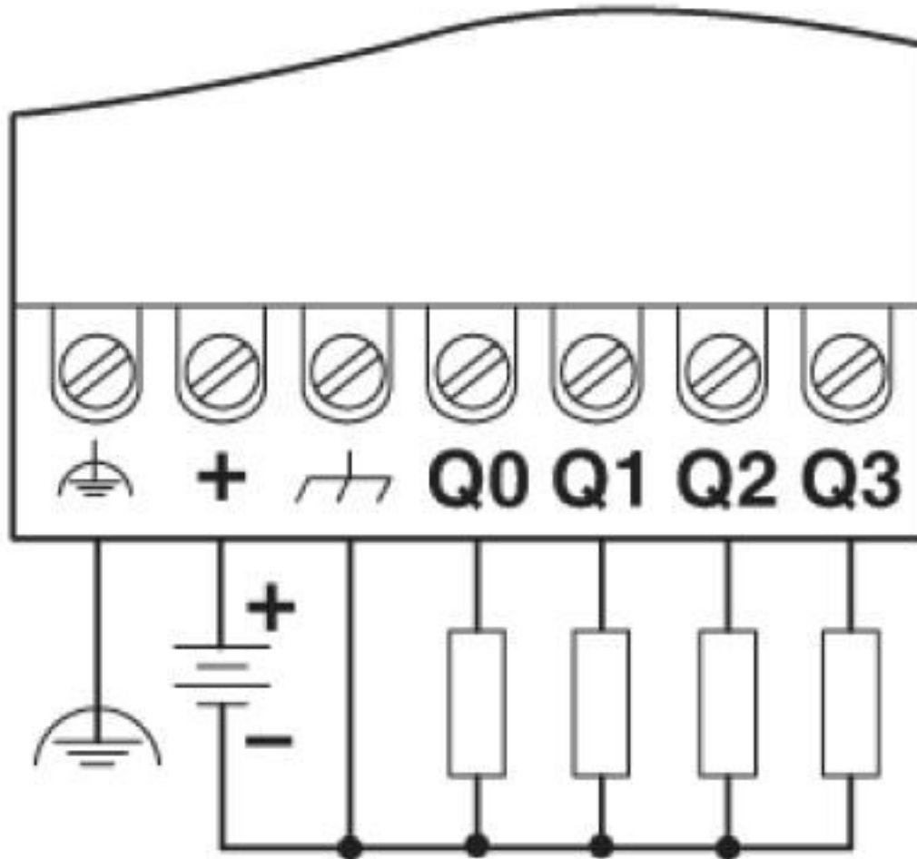
Connection diagram
