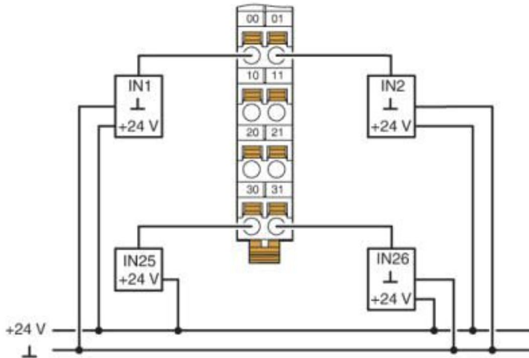
Connection diagram
