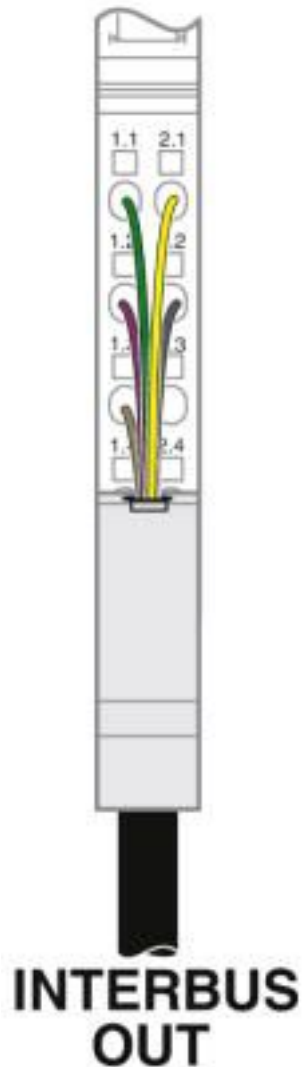
Connection diagram
