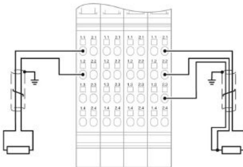
Connection diagram
