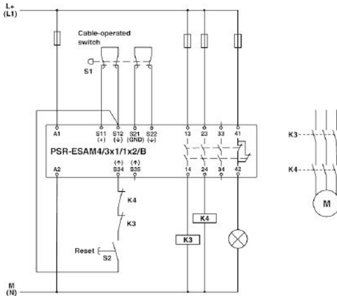
Cable-operated switch
