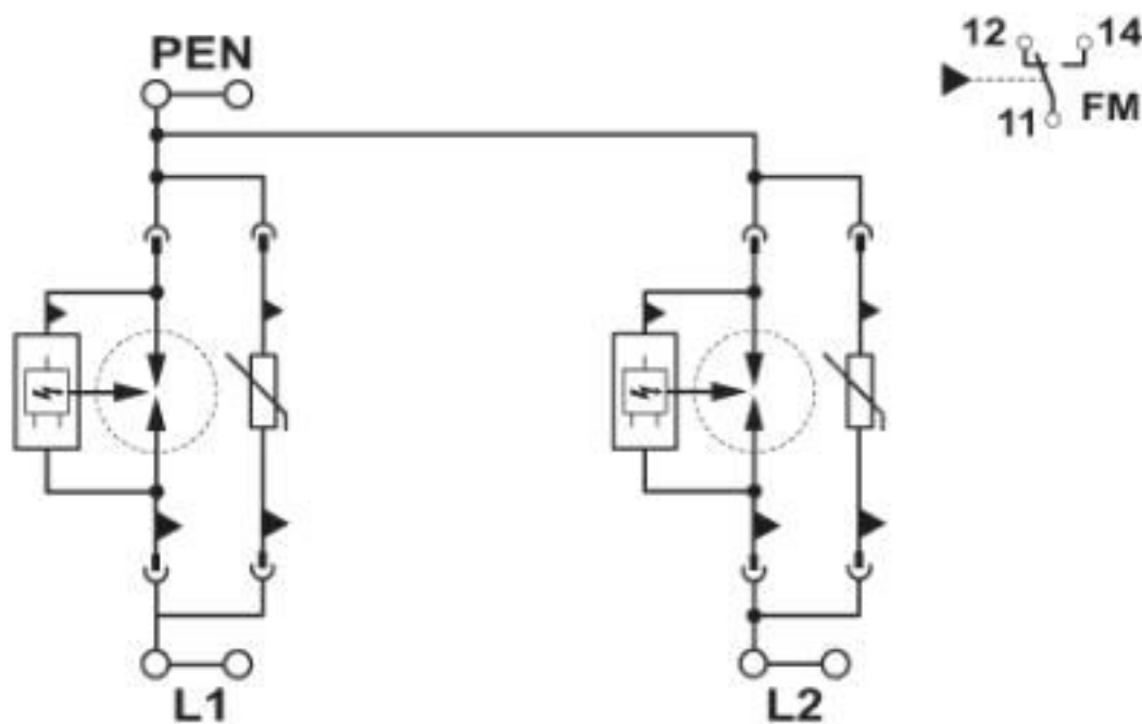
Circuit diagram
