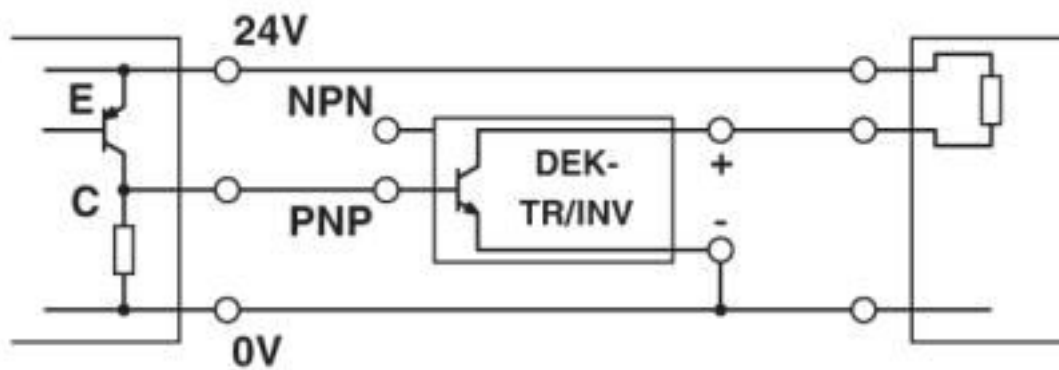
Application drawing
