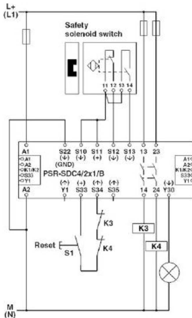
Circuit diagram
