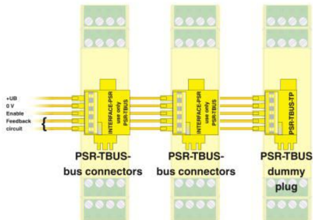
Connection diagram
