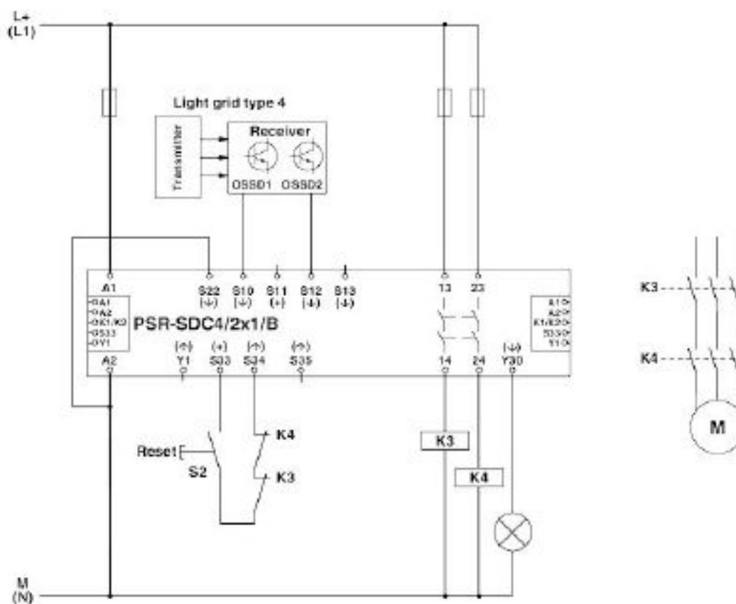
Circuit diagram
