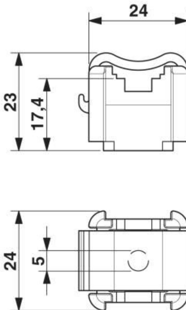
Dimensional drawing
