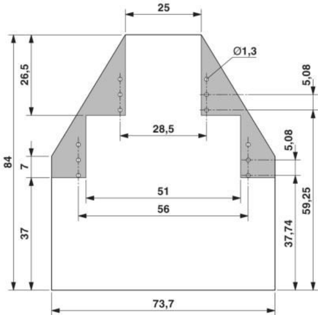
Dimensional drawing
