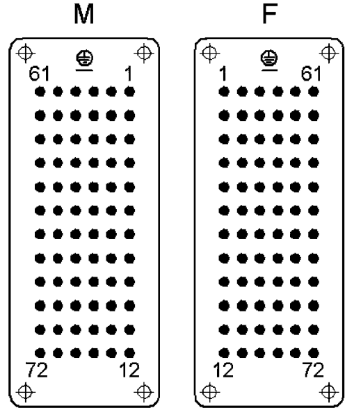
Pin Diagram, cable connection side
