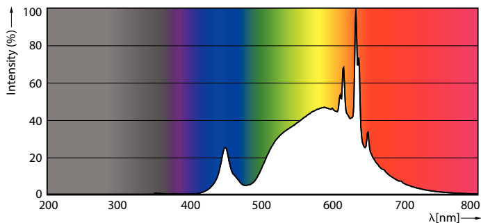
Spectral Power Distribution Colour - MAS LEDBulbND5.2-75W E27 830A70
