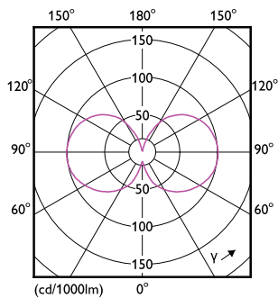
Light Distribution Diagram - MAS LEDBulbND5.2-75W E27 830A70 CLG UE
