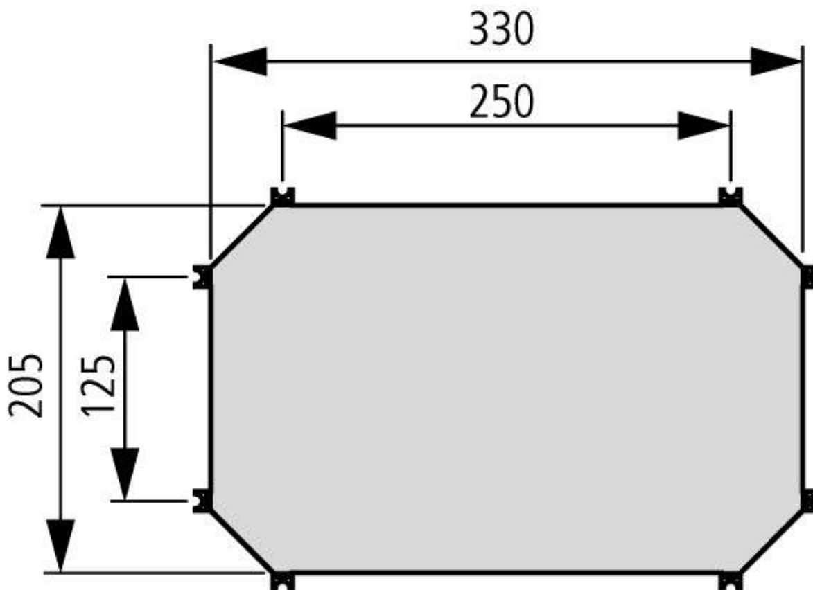
IM4... insulated mounting plate 4 mm thick
