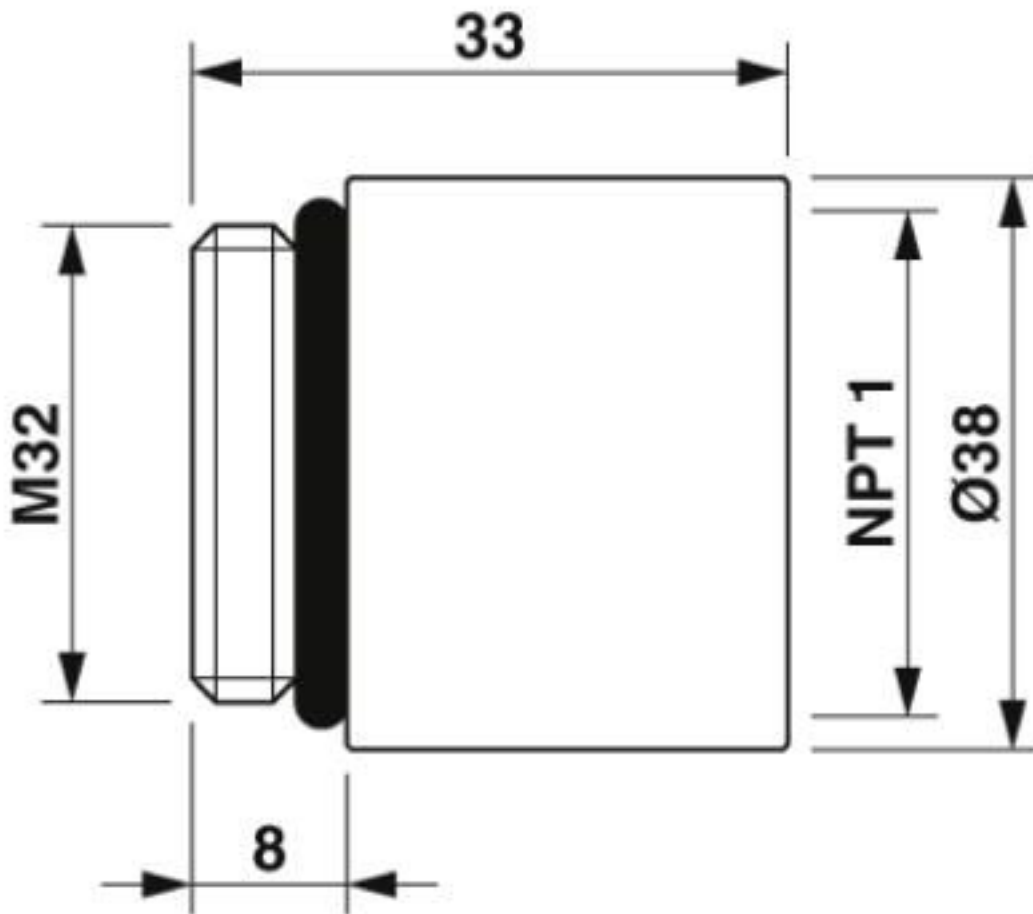
Dimensional drawing
