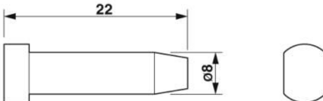
Dimensional drawing
